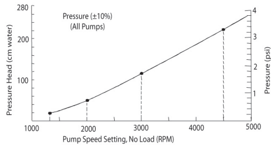
Pump Speed Setting vs. Pressure
